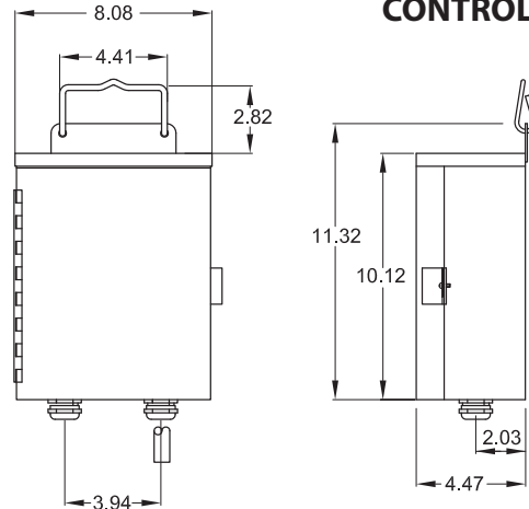
Control Box (1PH) 2H NEMA 3R - RAINPROOF CONTROL
